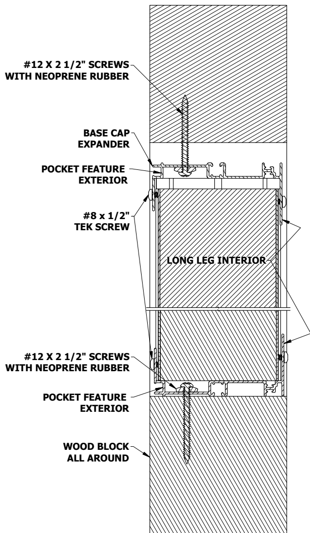
SECTION B-B
